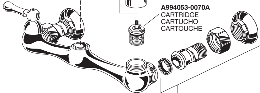
(OLD NUMBER) 014319-YYYOA (AFTER MAY, 1 2010) M962962-YYYOA FEMALE ECCENTRIC SHANK KIT KIT DE ESPIGA HEMBRA EXCENTRICA KIT DE QUEUE EXCENTRIQUE FEMELLE
